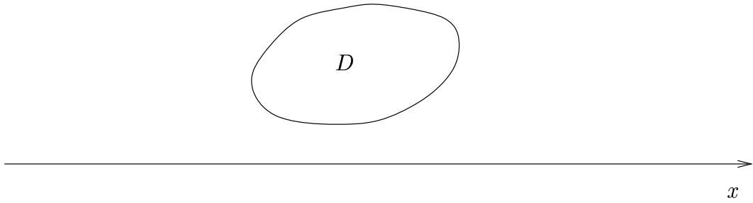
FIGURE 1. The scatterer D above the x -axis.
