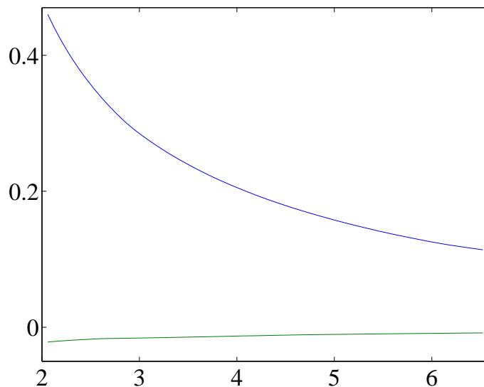
FIGURE 10. The maximum and minimum radiated energy through a segment as a function of distance r to the source (Example 4).
