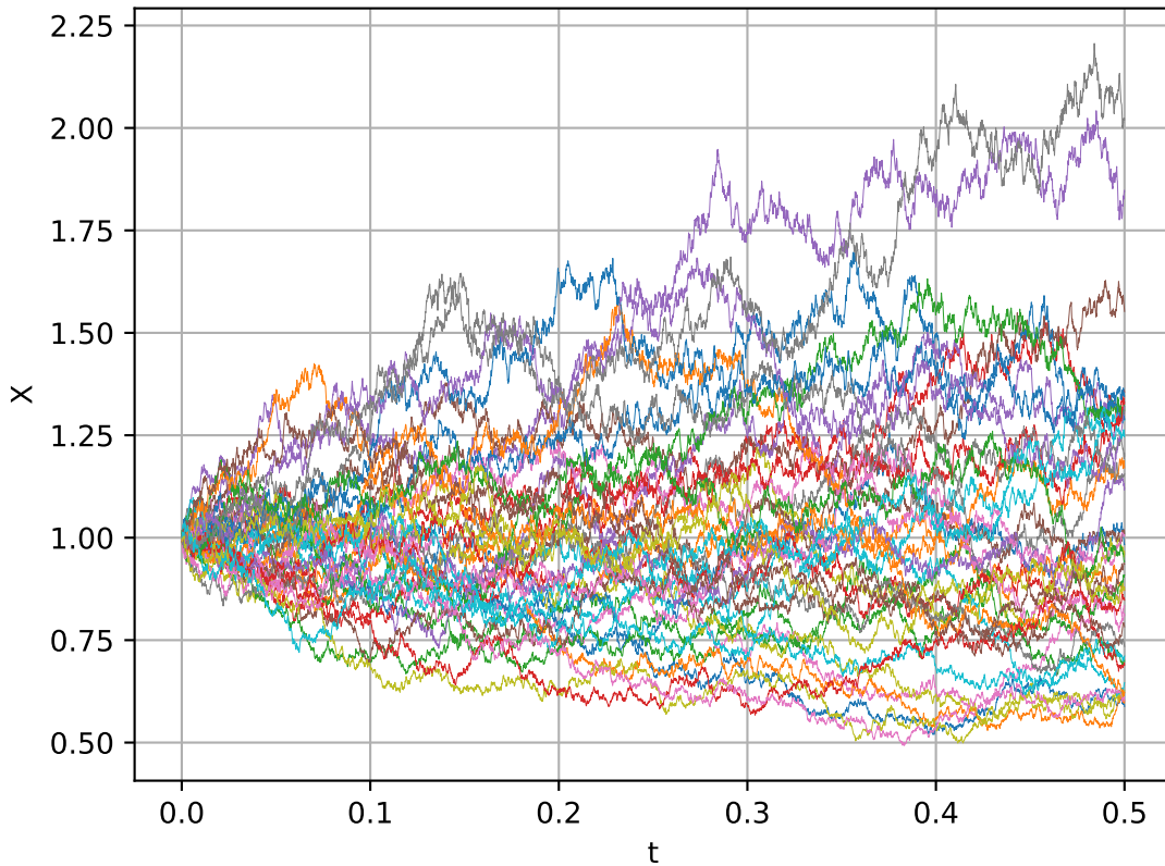
Geometric Brownian motion with sig=0.5, mu=0.2, dt=1.25e-04
