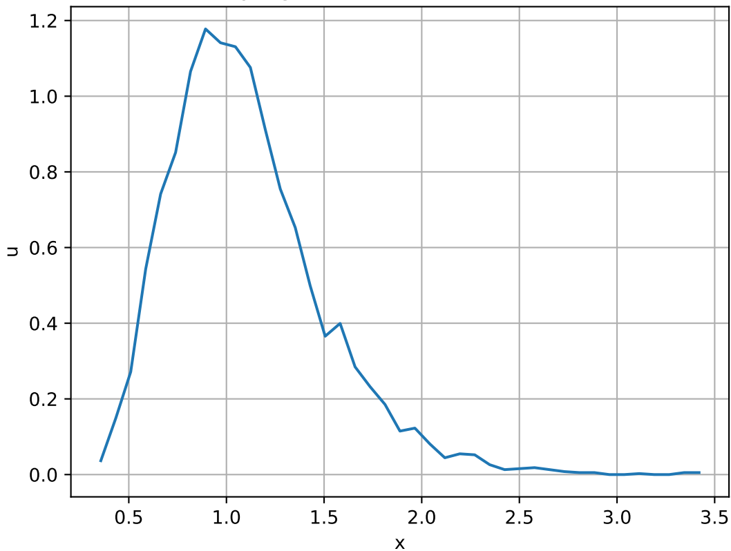
GBM density sig=0.5, mu=0.2, T=0.5, dt=1.25e-04
