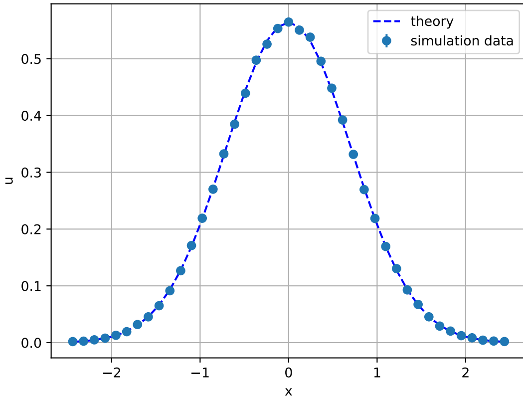
Sum of Gaussians, 3.00e+05 samples, 41 bins
