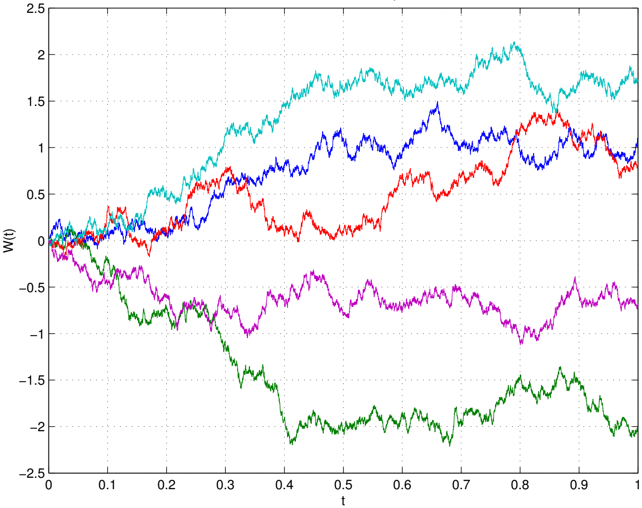
Five Brownian motion paths
