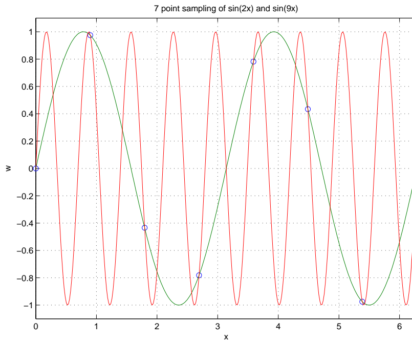
Figure 1: An illustration of aliasing with n = 7 sampling points and period p = 2\pi , with modes \alpha = 2 and \beta = \alpha + n = 9 . The continuous curves are \sin(2x) and \sin(9x) . The circles are these curves sampled at the sample points x_j = 2\pi j/n . The sampled values are identical even though the functions \sin(2x) and \sin(9x) are not.
