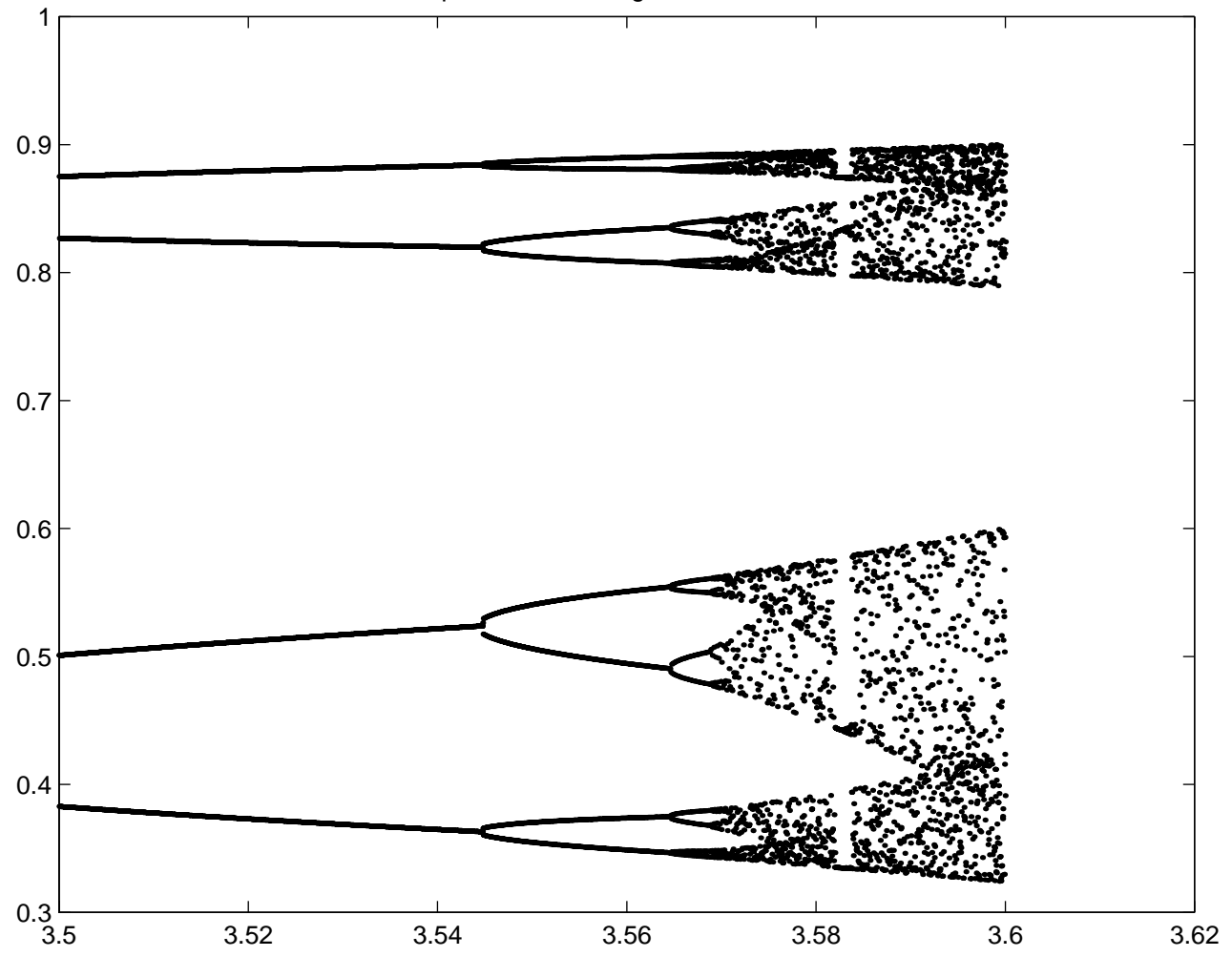
A picture of the Feigenbaum cascade
