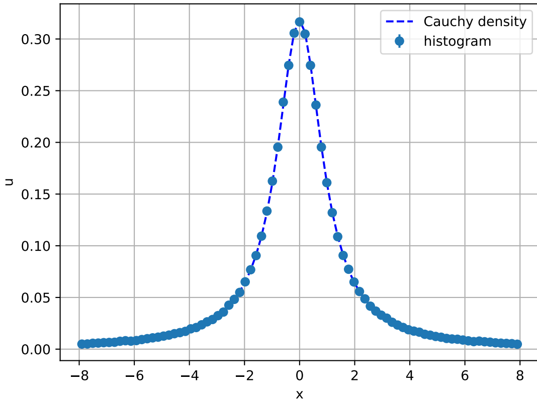
Cauchy density estimation, 1.00e+06 samples, 81 bins
