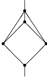
Figure 3: A graph vanishing in the quotient by the automorphism group.
