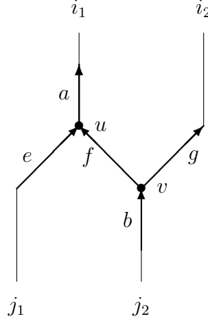
Figure 2: A configuration forbidden for \frac{1}{2} PROPs – f is a ‘bad’ edge. Vertices u and v might have more input or output edges which we did not indicate.
