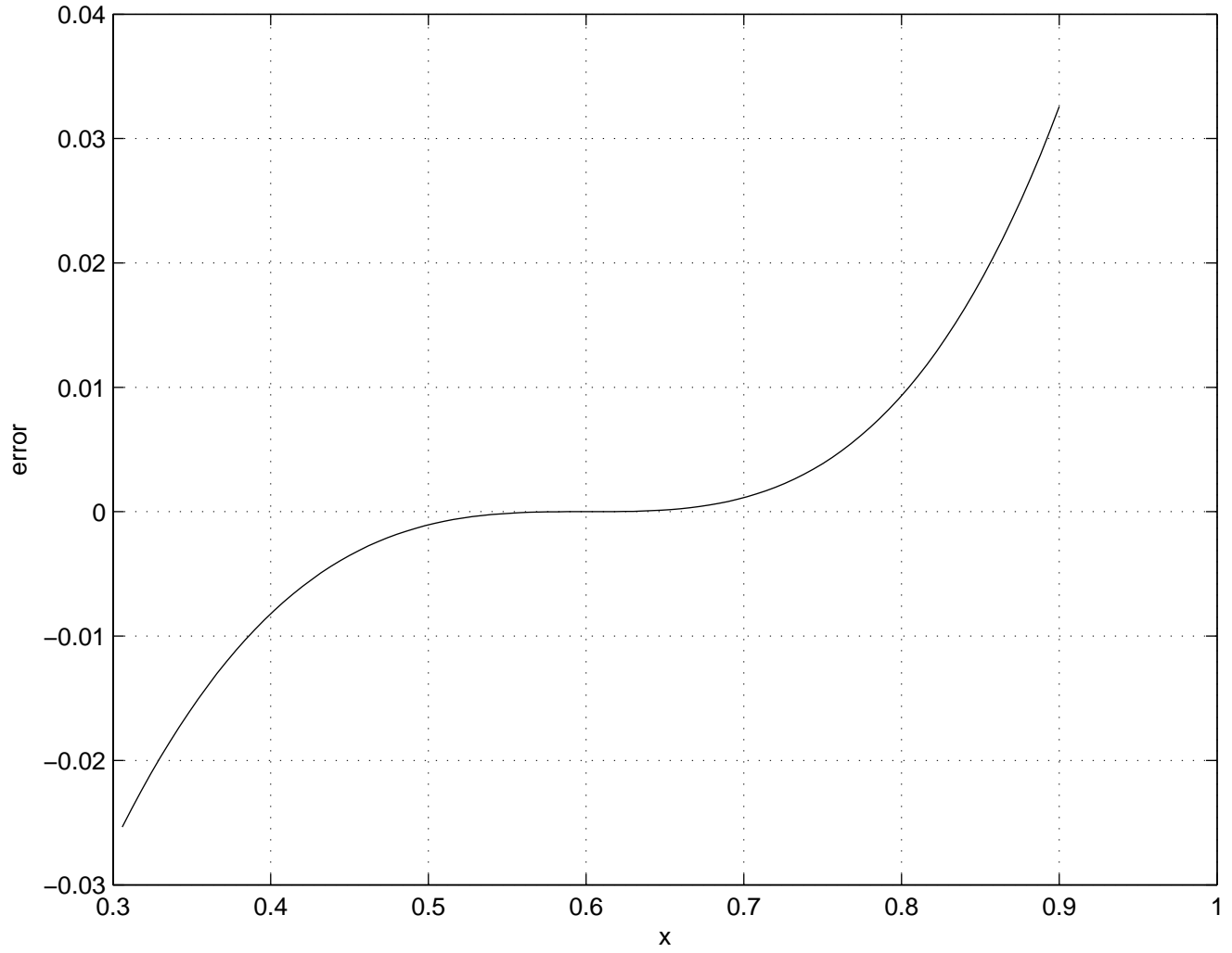
Error of the approximation of order two
