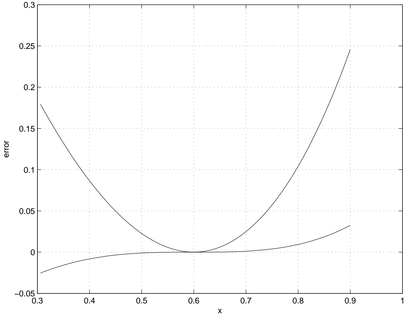
Errors of approximations of order one and two
