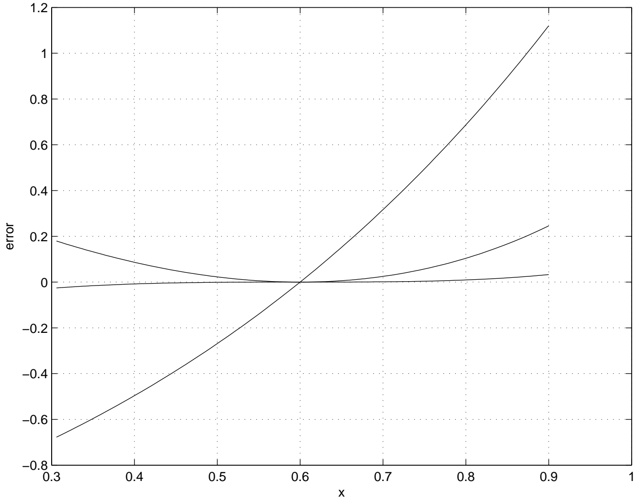
Errors of approximations of order zero, one, and two
