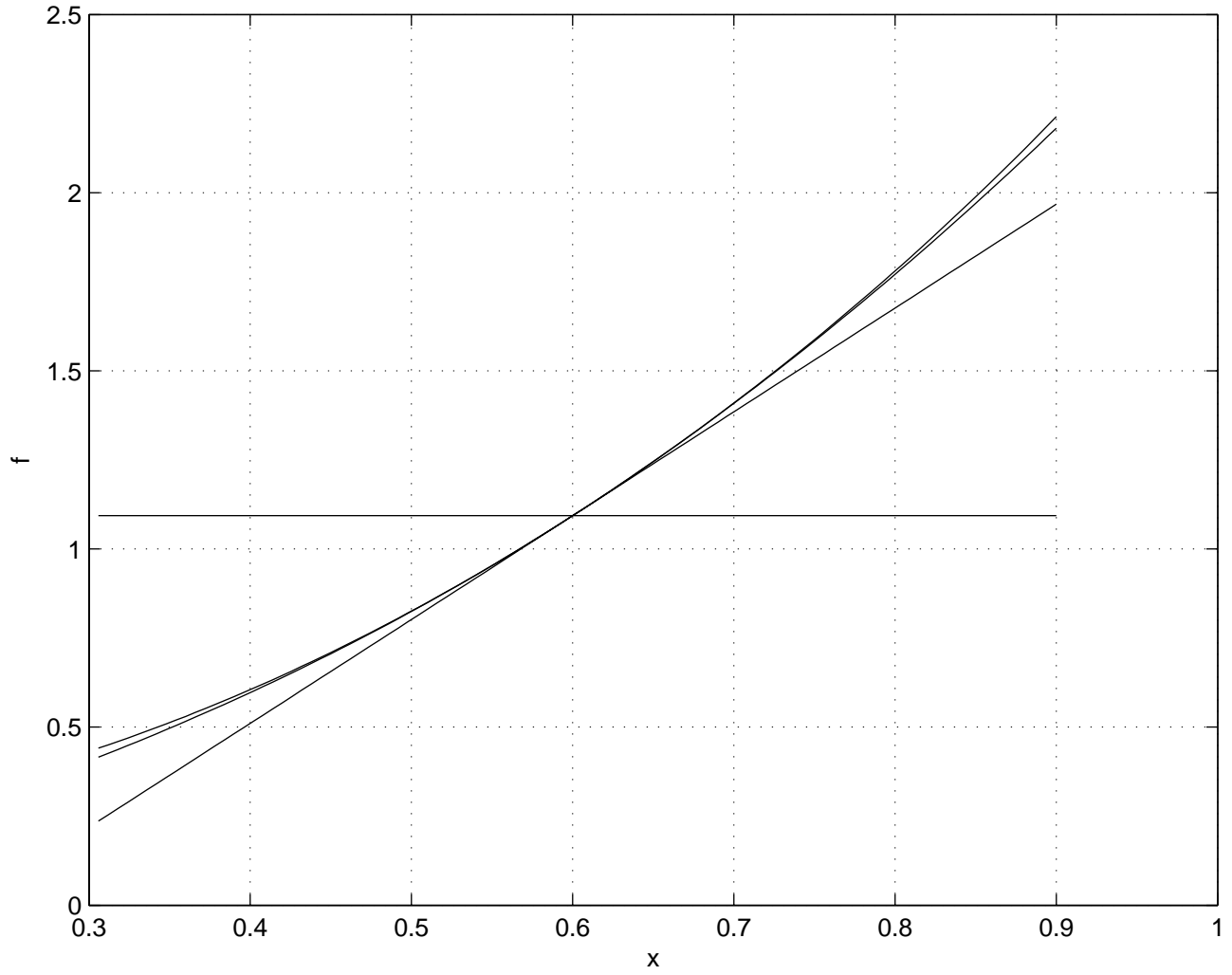
f(x) and approximations up to second order
