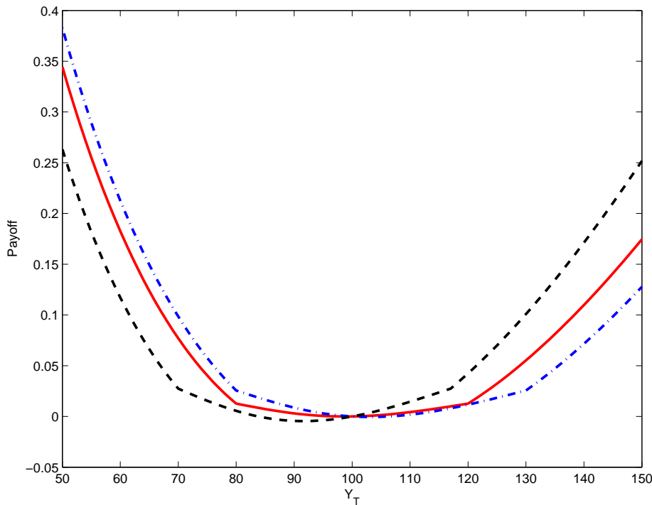
Fig. 4.1 Superreplicating portfolios for a variance call. Let Y_0 = 100 . A claim on any one of these time- T payoffs, together with dynamic trading of shares, model-independently superreplicates a spot-starting T -expiry variance call with strike Q = 0.04 . Referring to (4.1), the plots show L^*(Y_T) - L^*(Y_0) for three particular choices of (b_d, b_u) . Each superreplicating payoff is universally valid for all continuous semimartingales with Y_0 = 100 . The market prices of Europeans expiring at T determine which of the infinite family of superreplicating portfolios is cheapest; of course the cheapest need not be among these three examples.
