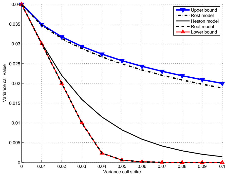
Fig. 5.1 Example: upper and lower bounds on a variance call. Let T = 1 . Given T -expiry European option prices consistent with the Heston model (5.1), the dynamics of Y are not uniquely determined. Three models of Y dynamics consistent with those prices are the Heston model itself, the Rost model, and the Root model, each of which generates a different profile of variance call values. We plot all three profiles, together with the lower bound V^{\text{SUB}} and upper bound V^{\text{SUPER}} derived, in (3.12) and (4.26), from the subreplicating and superreplicating hedges. The lower bound is, to the naked eye, indistinguishable from the Root model valuation (which is in fact larger than the lower bound at strikes 0.04 and higher, specifically larger by 0.3% at the ATM strike 0.04). The upper bound is nearly (within 2.6% at the ATM strike 0.04) attained by the Rost model.
