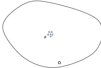
Figure 2: Minimizers with small number of vortices.
