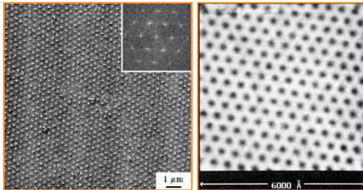
Figure 1: Abrikosov lattices, H. F. Hess et al. Phys. Rev. Lett. 62, 214 (1989).
