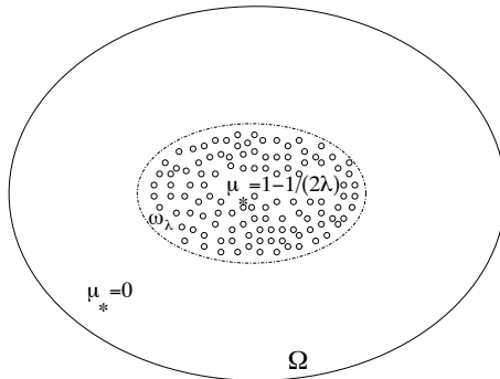
Figure 4: Optimal density of vortices according to the obstacle problem.
