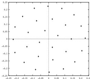
Figure 3: Numerical minimization of H_n by Gueron-Shafrir [GS], n = 29 .
