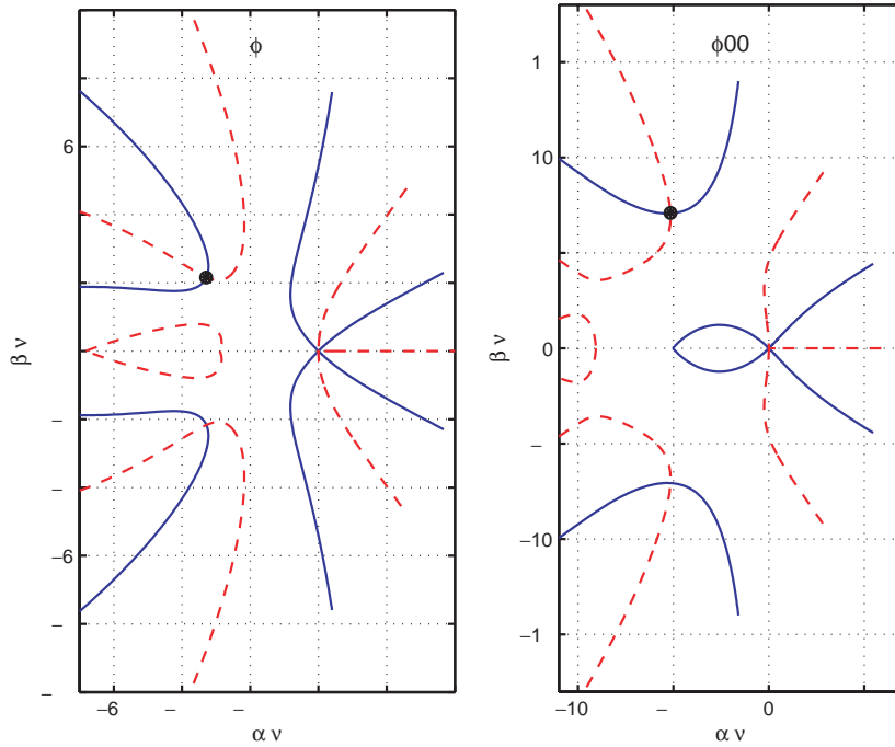
FIG. 7.1. Zero-level contours of \mathcal{D}(\Omega_o; \phi, p) for p = 3 and two values of \phi . The solid lines correspond to the real part and the dashed lines to the imaginary parts. Intersection points represent the natural modes of oscillation of the fiber.
