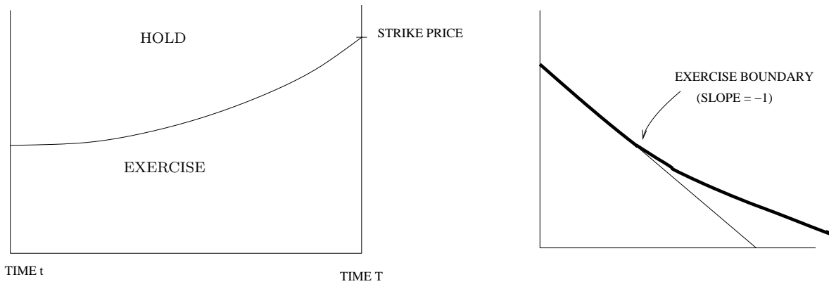
Figure 2: The exercise boundary of an American option, and its value as a function of stock price at a given time t
