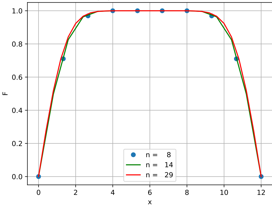
Value function for payout at time 1.25 with lambda = 0.50
