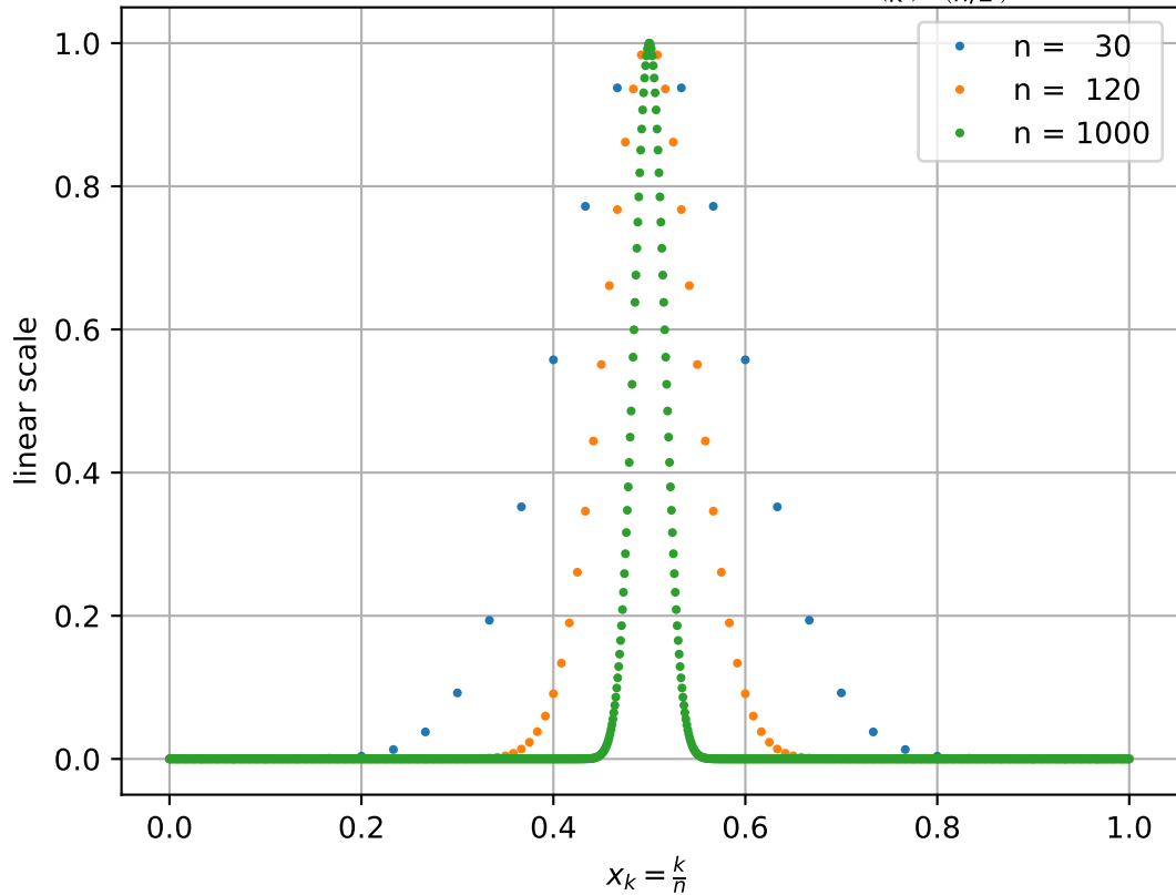
Normalized binomial coefficients \binom{n}{k} / \binom{n}{n/2}
